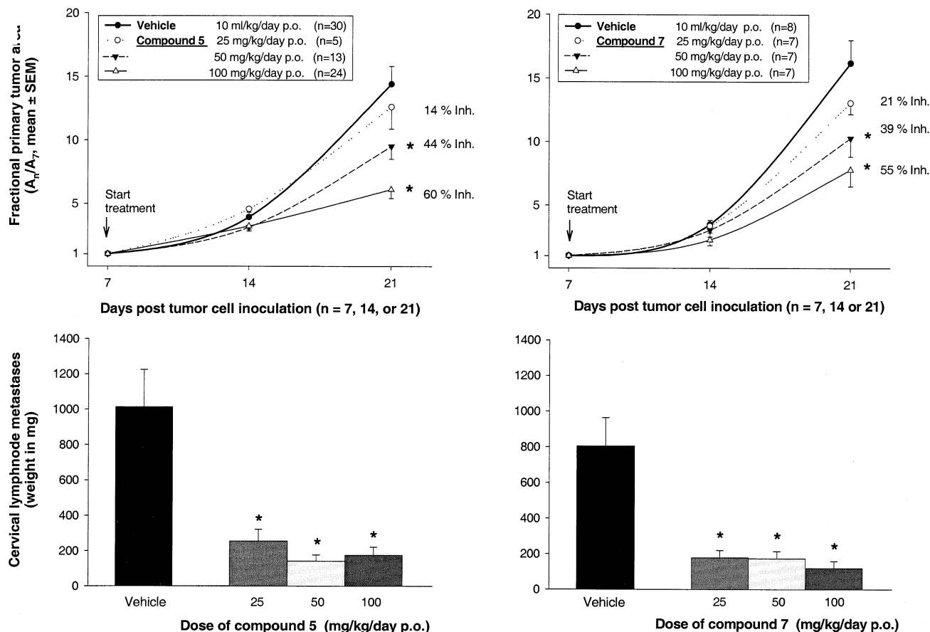
Figure 2. Dose-dependent antitumor and antimetastatic effects of compounds 5 (left) and 7 (right) in a B16/BL6 melanoma orthotopic model in C56BL/6 mice after oral administration. Dose-response effects on primary tumor growth are expressed in terms of relative mean tumor area quantified on day 14 ( A_{14} ) and day 21 ( A_{21} ) after intradermal injection into the ears, compared to that on day 7 ( A_7 ), and are shown in the upper panels; percent inhibition on day 21 (14 days treatment) is given for each curve. Absolute tumor mean areas at day 7 ( A_7 ) were in the range 0.97 \pm 0.09 to 1.42 \pm 0.13 mm 2 and not statistically different. The influence of the compounds on cervical lymph node metastases, quantified by the weight of the cervical lymph nodes after surgical removal, are shown in the panels below. Values are mean \pm SEM, * P < 0.5 , ANOVA, Dunns, significance compared to vehicle-treated group.
